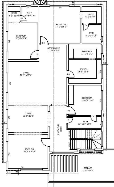
FIRST FLOOR PLAN SCALE: 1/8"=1'-0"
