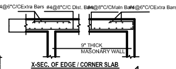
X-SEC. OF EDGE / CORNER SLAB
