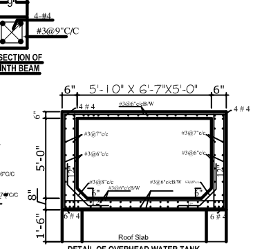
DETAIL OF OVERHEAD WATER TANK 5'-10" X 6'-7" X 5'-0"
