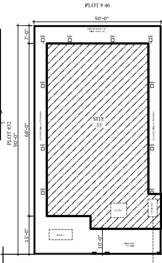
STREET # 1 40'-0" WIDE
