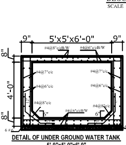
DETAIL OF UNDER GROUND WATER TANK 5'-0" X 5'-0" X 6'-0"
