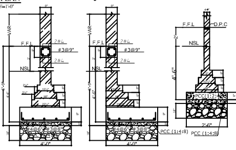
DETAIL OF FOUNDATIONS SCALE: 1/8"=1'-0"
