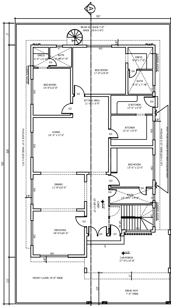
GROUND FLOOR PLAN SCALE: 1/8"=1'-0"
