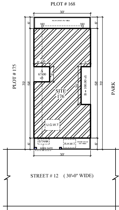
SITE PLAN
