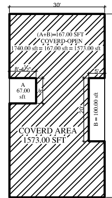
GROUND FLOOR BLOCK PLAN
