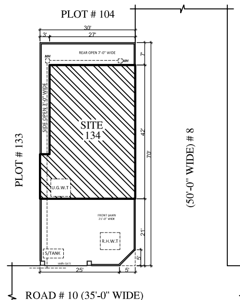
SITE PLAN SCALE 1/16"=1'-0"
