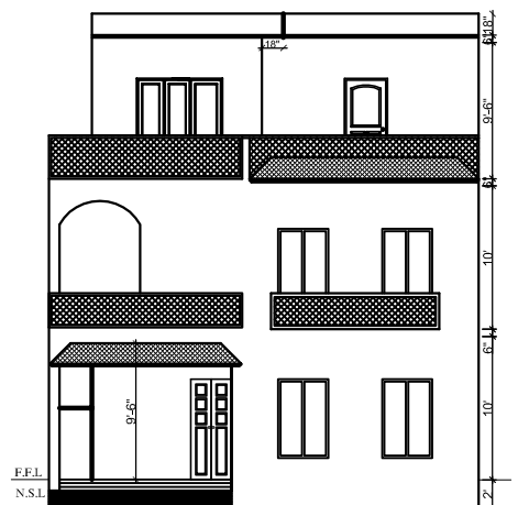
FRONT ELEVATION Scale 1/8"=1'-0"
