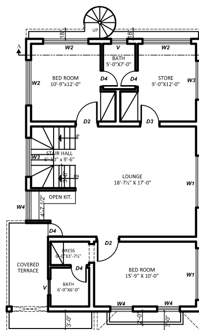
FIRST FLOOR PLAN SCALE 1/8"=1'-0"
