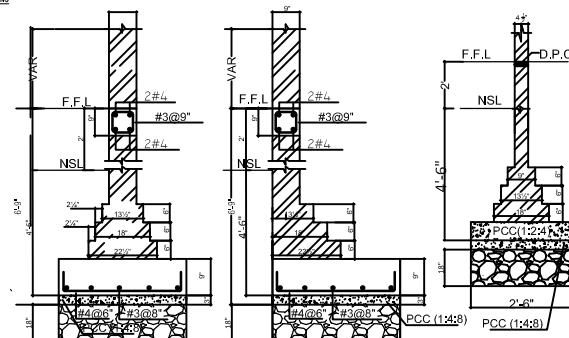
DETAIL OF FOUNDATIONS
