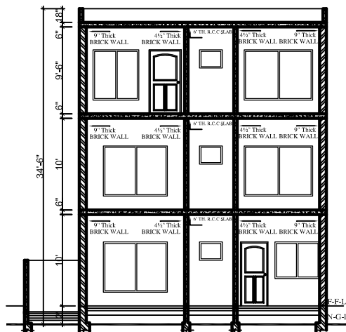
SECTION AT (A-A) Scale 1/8"=1'-0"
