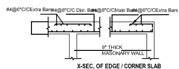
X-SEC. OF EDGE / CORNER SLAB
