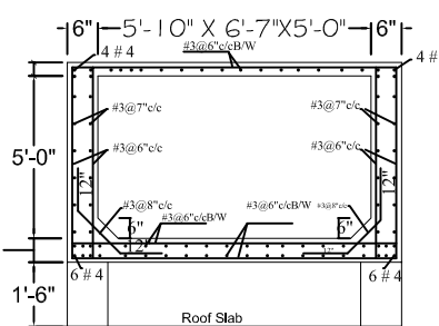
DETAIL OF OVERHEAD WATER TANK 5'-10" X 6'-7" X 5'-0"
