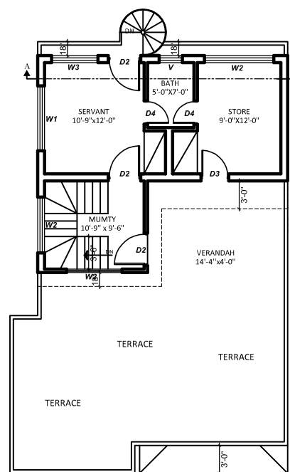
MUMTY FLOOR PLAN SCALE 1/8"=1'-0"
