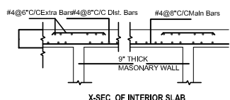
X-SEC. OF INTERIOR SLAB
