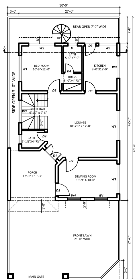
GROUND FLOOR PLAN SCALE 1/8"=1'-0"
