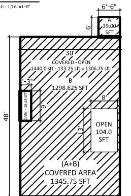
GROUND FLOOR BLOCK PLAN
