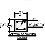
X-SECTION OF CONFINED COLUMN
