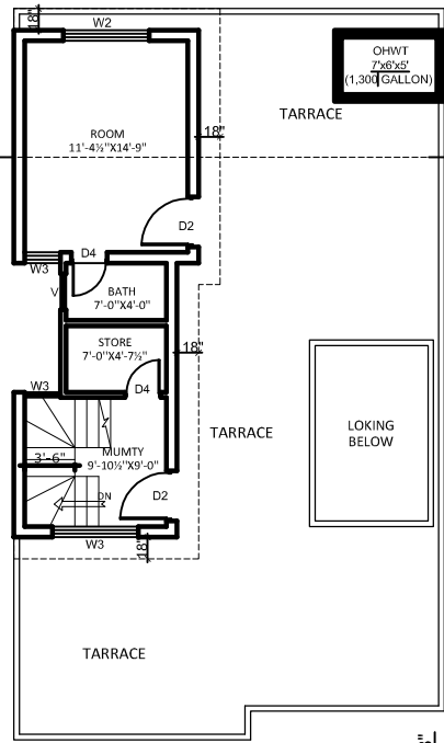
MUMTY FLOOR PLAN
