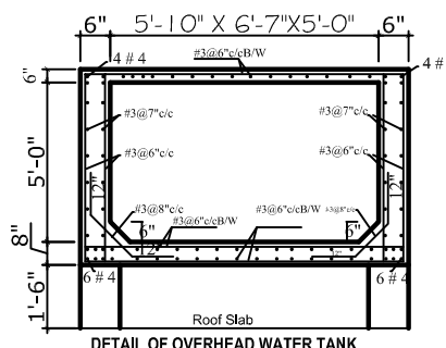
DETAIL OF OVERHEAD WATER TANK
