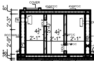
DETAIL OF DISPOSAL
