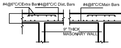
X-SEC. OF INTERIOR SLAB
