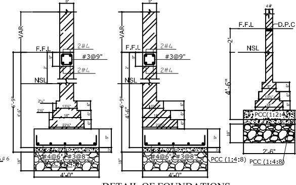
DETAIL OF FOUNDATIONS
