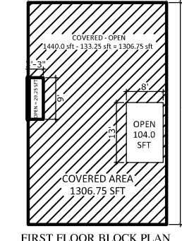
FIRST FLOOR BLOCK PLAN
