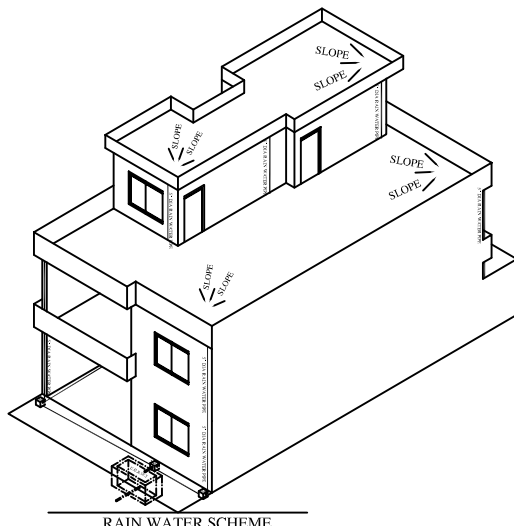
RAIN WATER SCHEME
