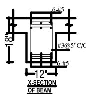
X-SECTION OF BEAM
