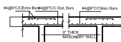
X-SEC. OF INTERIOR SLAB
