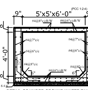
DETAIL OF UNDER GROUND WATER TANK
