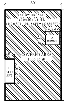
FIRST FLOOR BLOCK PLAN
