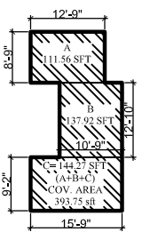
MUMTY FLOOR BLOCK PLAN
