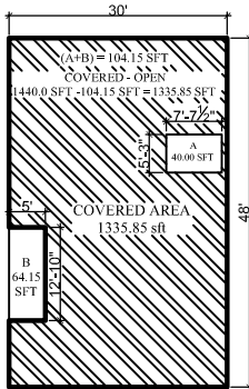
GROUND FLOOR BLOCK PLAN
