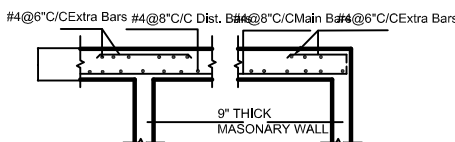
X-SEC. OF EDGE / CORNER SLAB
