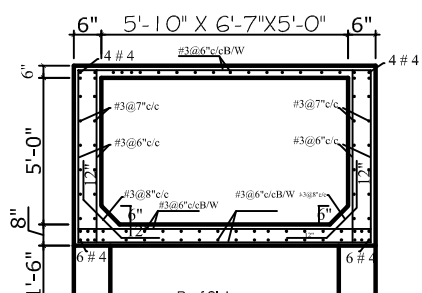
DETAIL OF OVERHEAD WATER TANK
