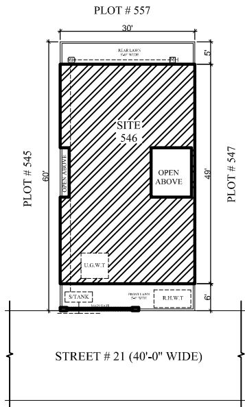
SITE PLAN SCALE 1/16"=1'-0"
