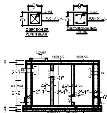
DETAIL OF DISPOSAL 7'-0"X4'-0"X5'-0"
