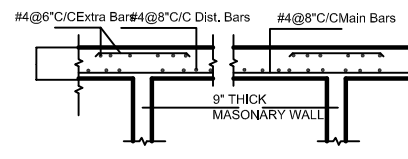
X-SEC. OF INTERIOR SLAB
