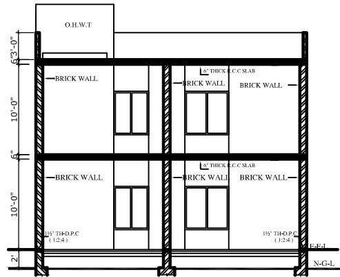
SECTION AT A-A Scale 1/8"=1'-0"
