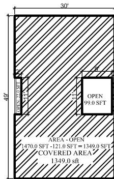
FIRST FLOOR BLOCK PLAN SCALE 1/16"=1'-0"
