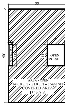
GROUND FLOOR BLOCK PLAN SCALE 1/16"=1'-0"
