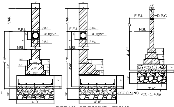
DETAIL OF FOUNDATIONS SCALE: NTS
