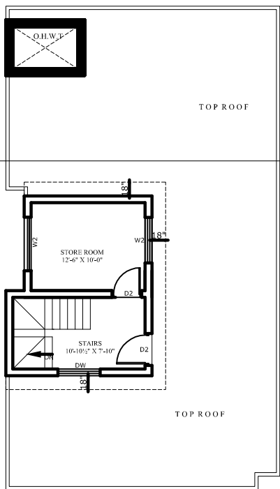
MUMTY FLOOR PLAN SCALE : 1/8"=1'-0"
